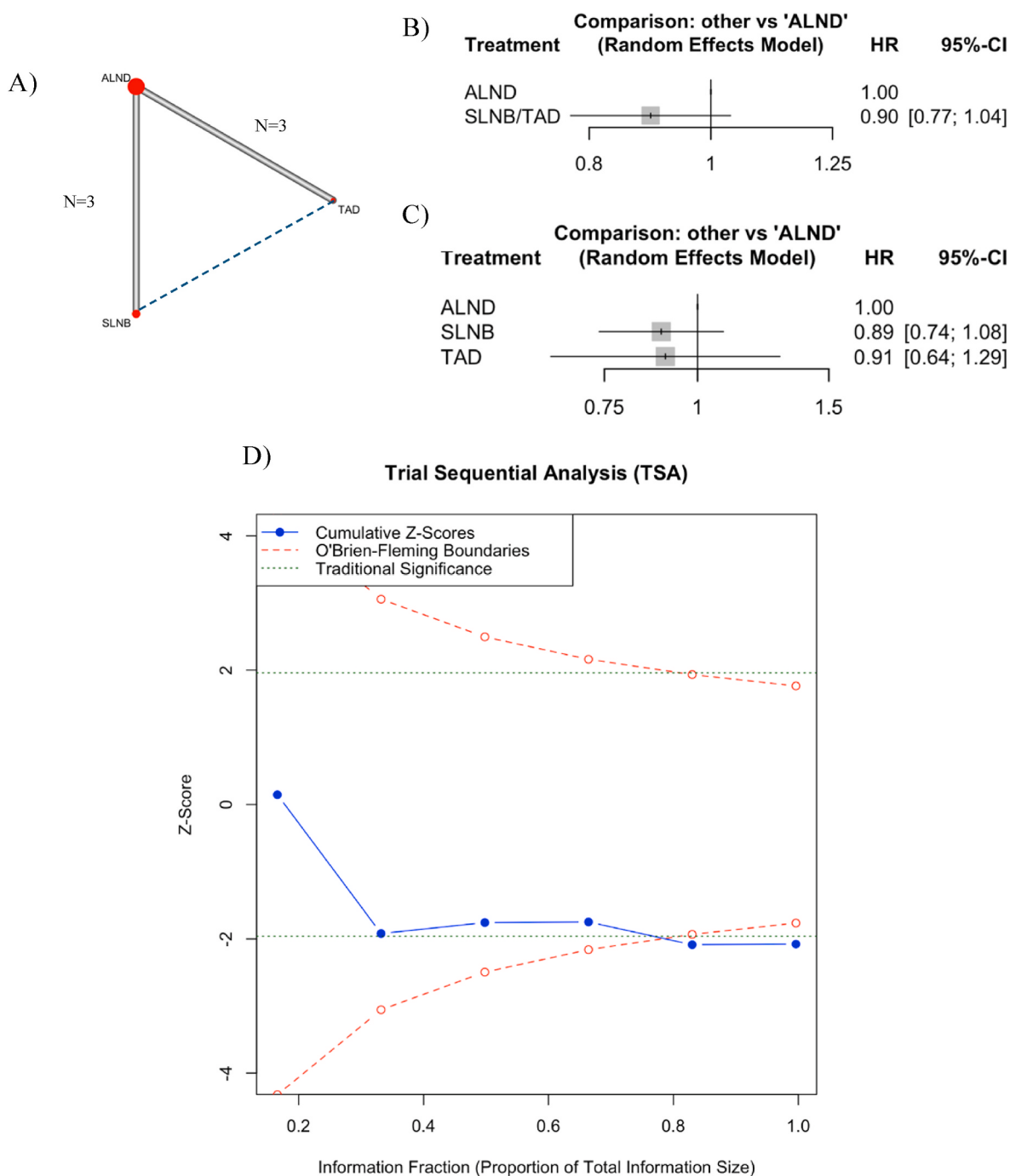
Fig. 5. A) Network plot of studies comparing DFS; B) and C) Direct comparisons of DFS between SLNB/TAD versus ALND D) TSA of studies comparing DFS.
