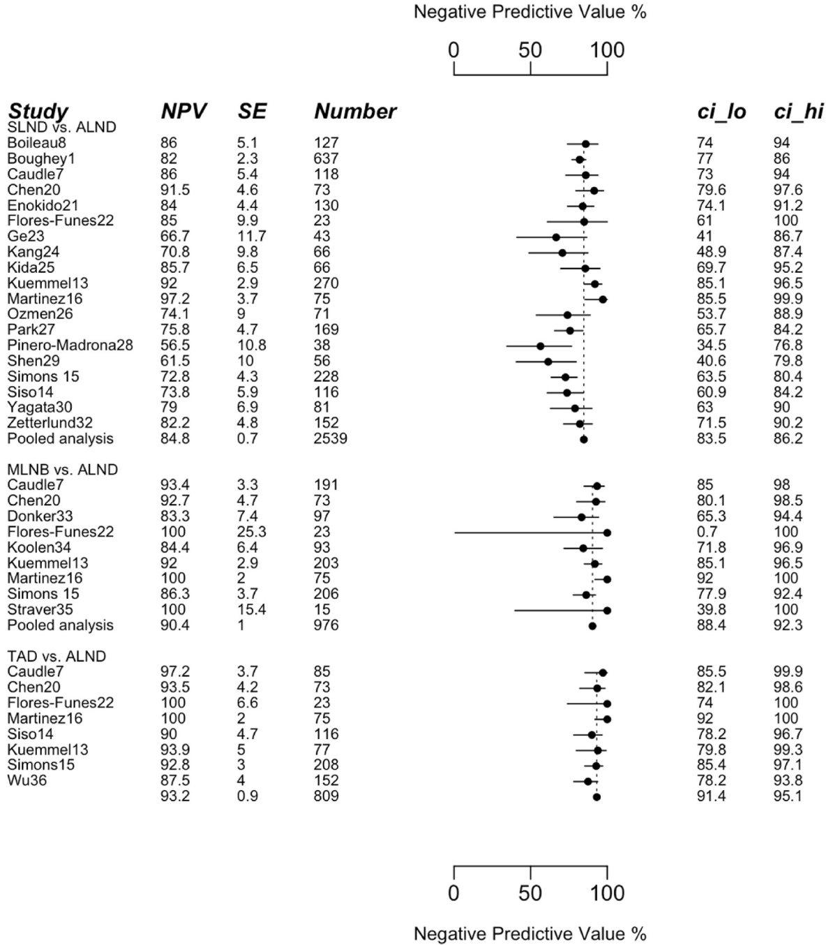
Fig. 4. NPV of SLNB, MLNB and TAD compared to reference ALND.
