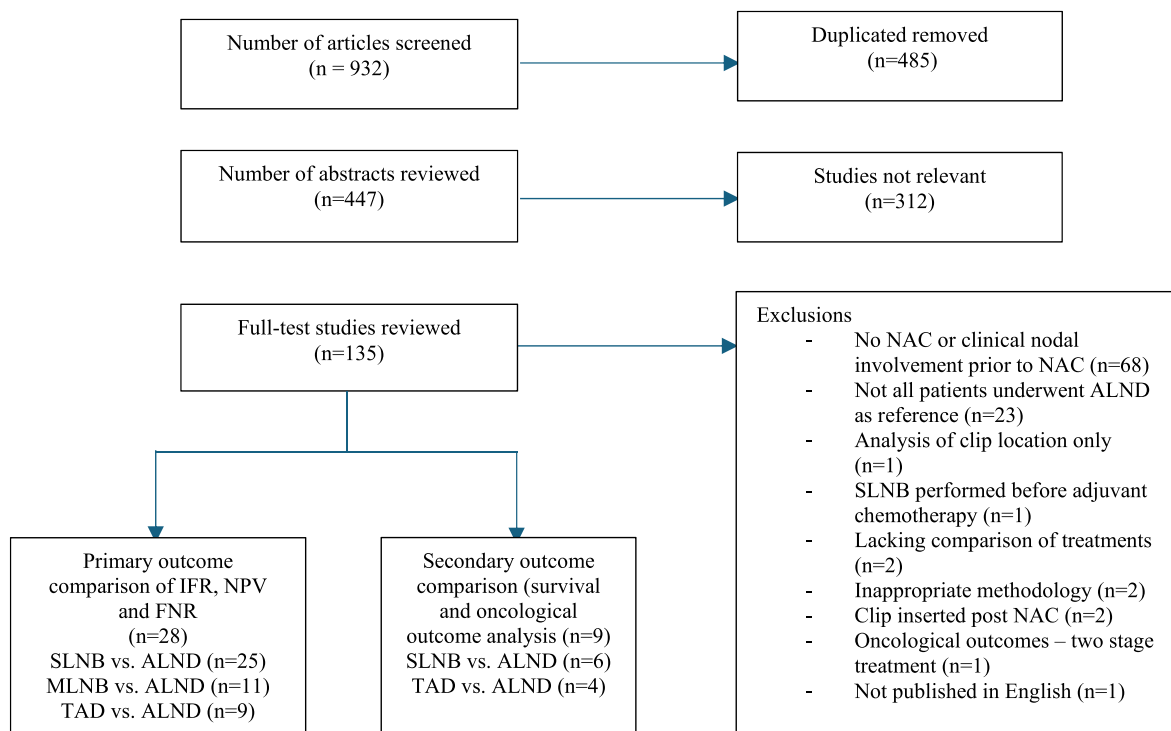
Fig. 1. PRISMA-flow diagram.
