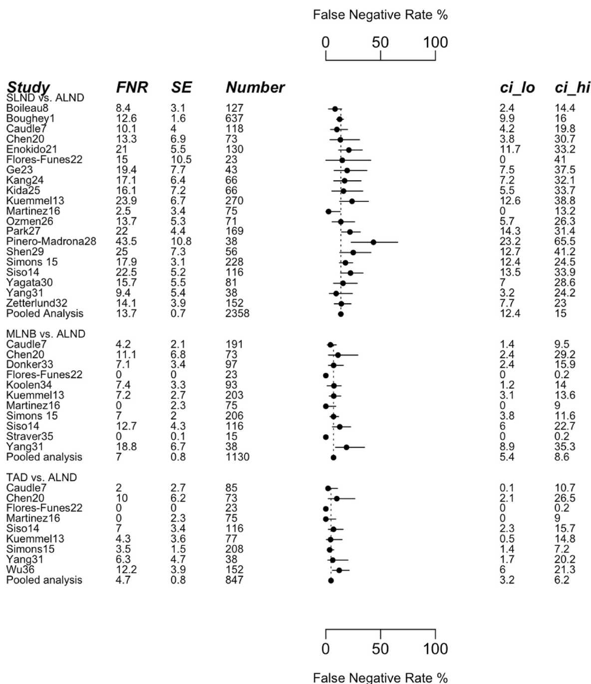
Fig. 3. FNR of SLNB, MLNB and TAD compared to reference ALND.
