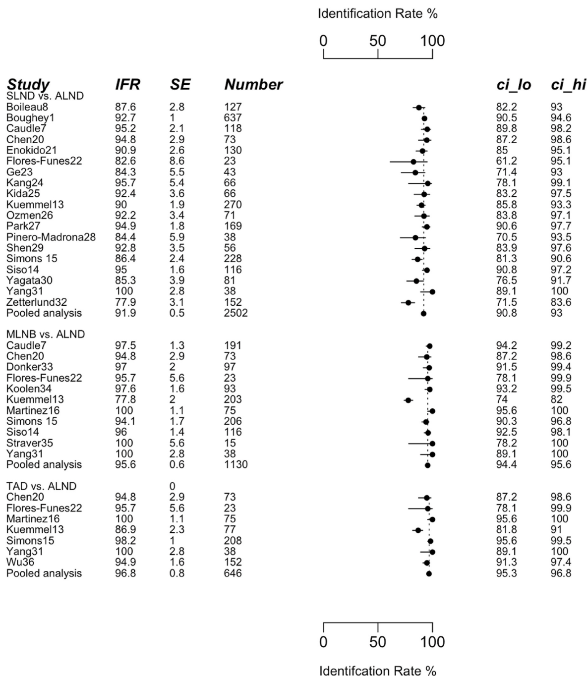
Fig. 2. IFR of SLNB, MLNB and TAD compared to reference ALND.
